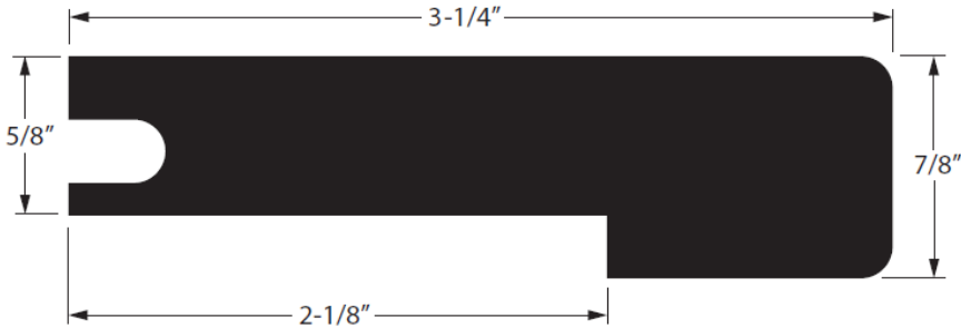
Stair Nose (038)
