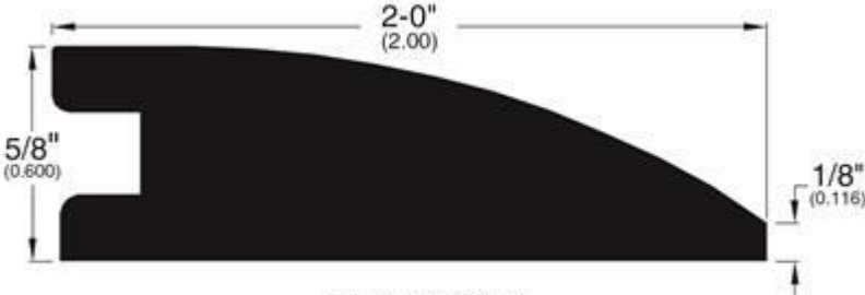
Reducer (037)
