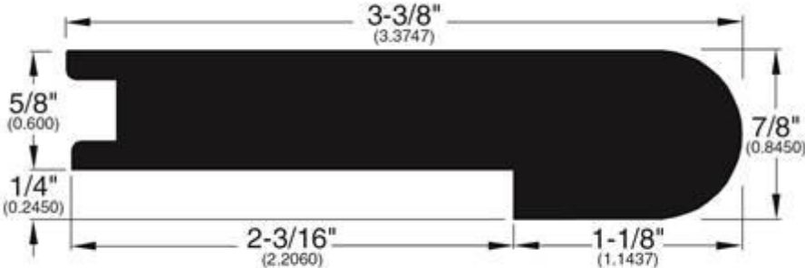
Stair Nose (038)
