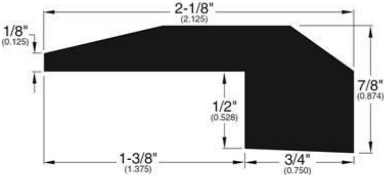
Threshold (011)
