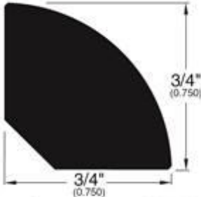
Quarter Round (001)
